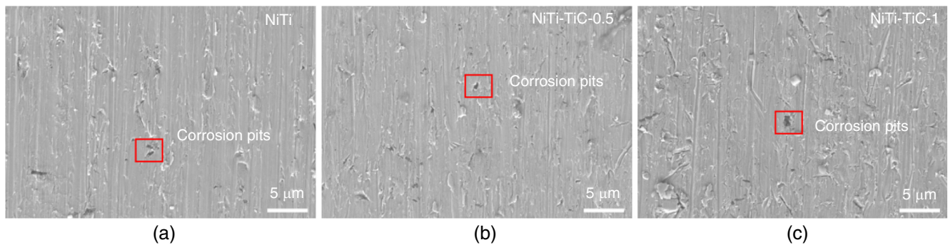
FIGURE S1. The SEM images after corrosion of (a) NiTi, (b) NiTi-TiC-0.5 and (c) NiTi-TiC-1
